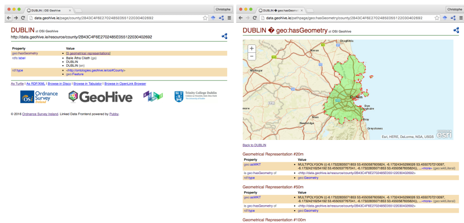
Fig. 1. Description in HTML of County Dublin on the left and its three geometries – with the one generalized up to 100 meters drawn on a map – on the right.
