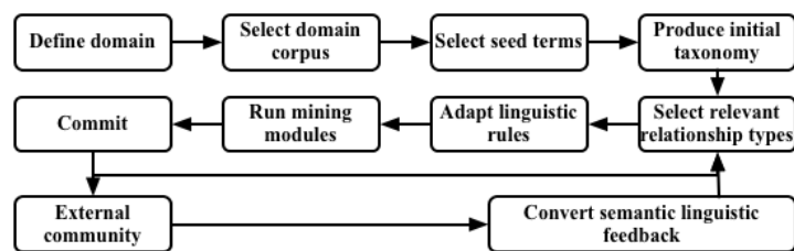
Fig. 2. A general view of the MTB process: ontological and other updates from the external community are taken over to perform a new mining and modeling cycle. The Termino Platform supports humans through different steps. The mining modules in the middle of the process use the incoming rules, predefined seed terms and statistic criteria to extract possible terminological and ontological-relevant information that terminologists validate for internal and external consumption.
