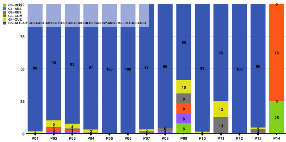
Fig. 4. The discussion effort distribution per actor leads to identification of initiative takers (REQ), answers (ANS), and spammers (RES, REQ; but nothing else).
